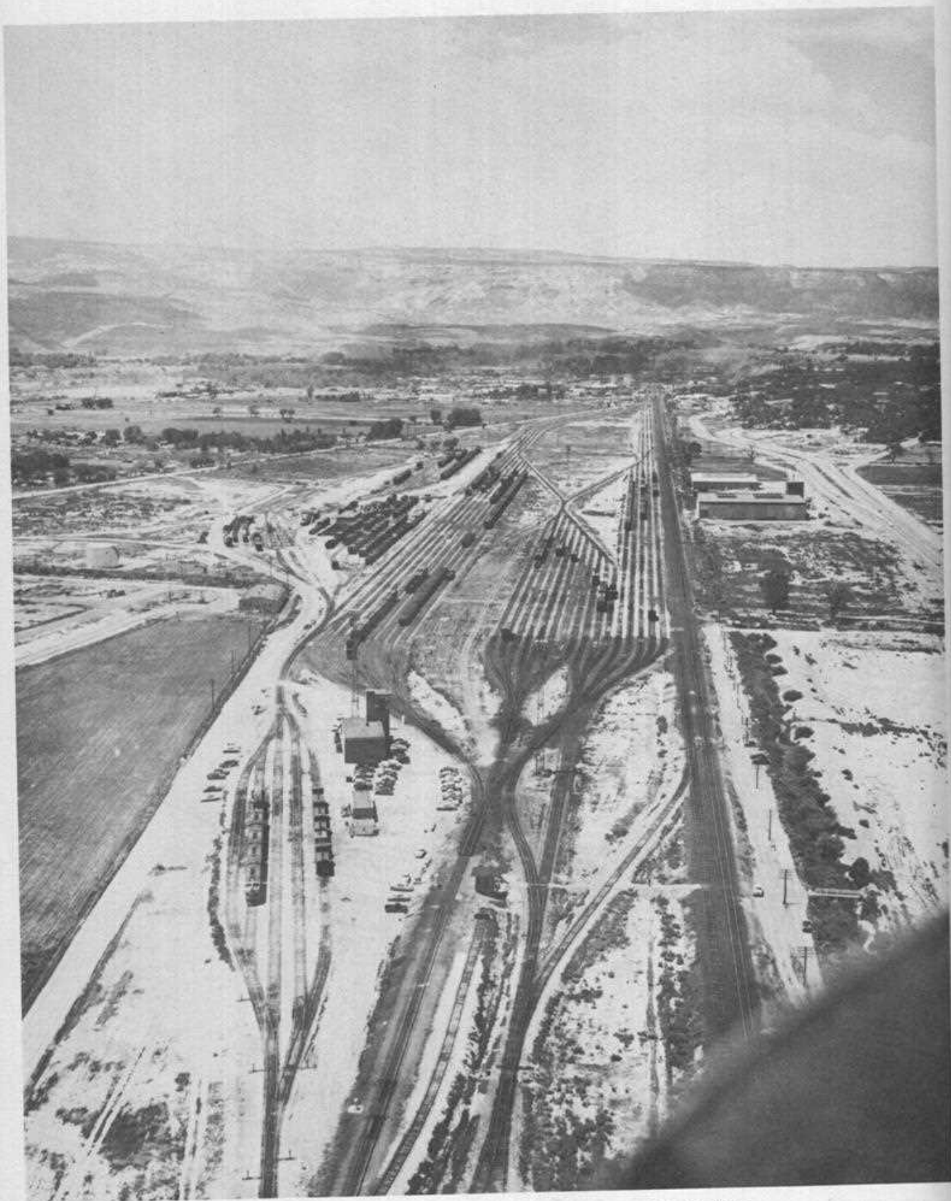
GRAND JUNCTION CLASSIFICATION YARD
